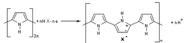
Fig. 1. Doping mechanism of PPy [5]
