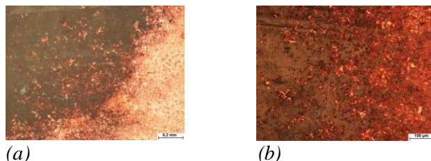
Fig.4 – Microscope photos of the copper front (a) x50 (b) x100
