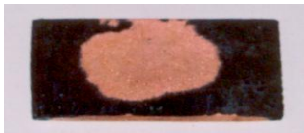
Fig. 5 – Photograph of a specimen during the copper electroplating
