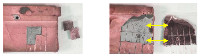
Fig. 7 – ASTM D 3359, method B test on copper plated ABS/PPy electrodes.
